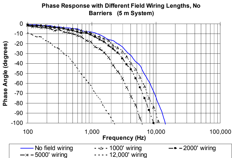
Figure 10 Frequency Response, typical 3300 XL 8 mm 5 m System with varying lengths of field wiring attached, no barriers
