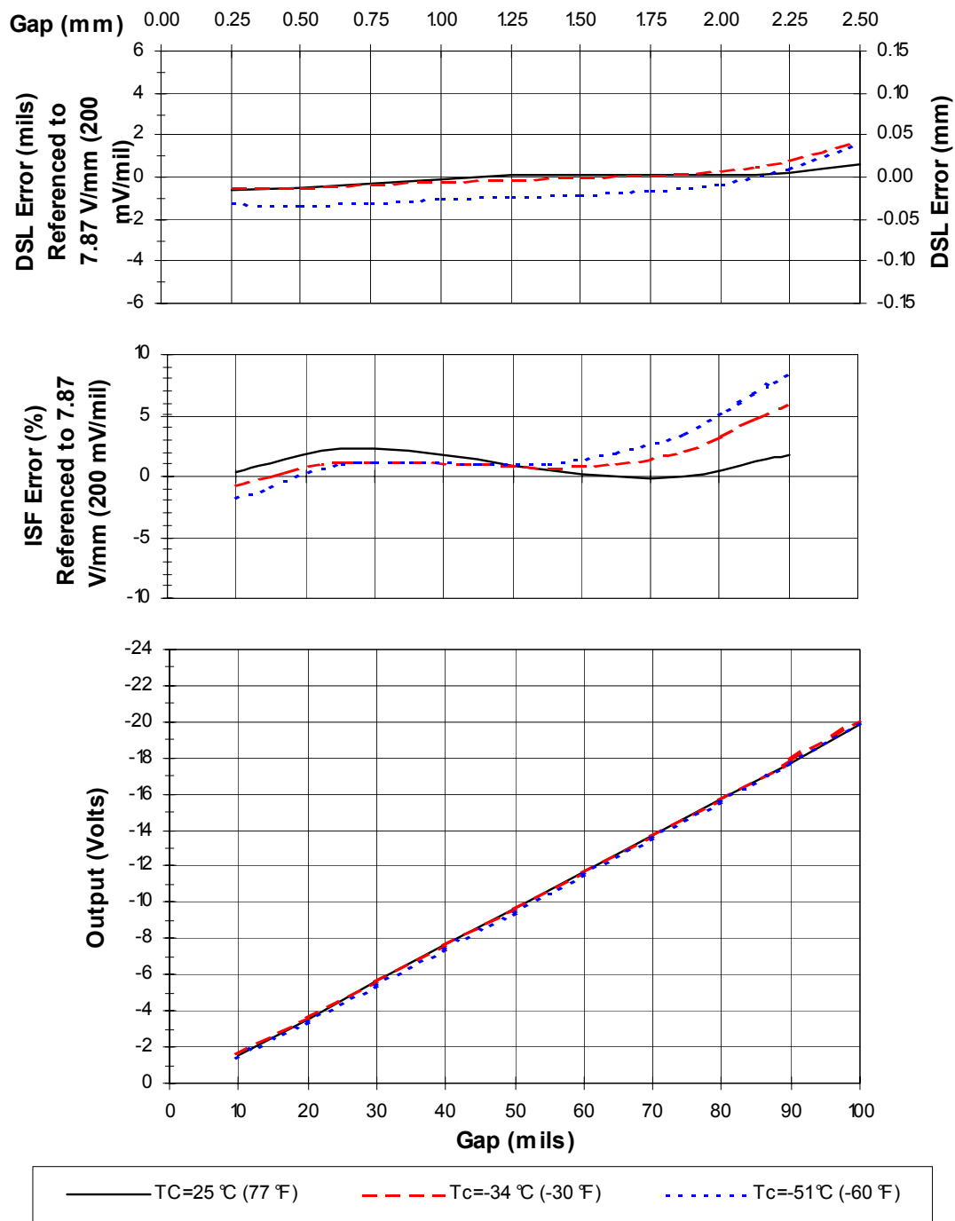
Figure 4 Typical 3300 XL 8 mm 5 m Proximity® Sensor with 4 m of Extension Cable @ Tc (Probe is at 25 °C)
